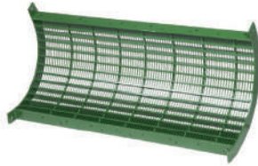
CONCAVE (4 STRAW WALKER)
